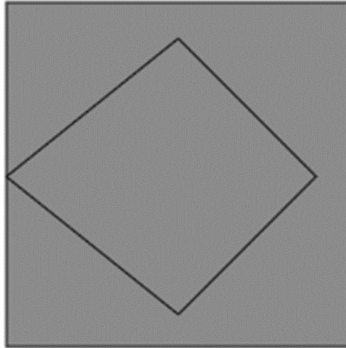
31. Use of D02 to start an new overlapping and touching contour
