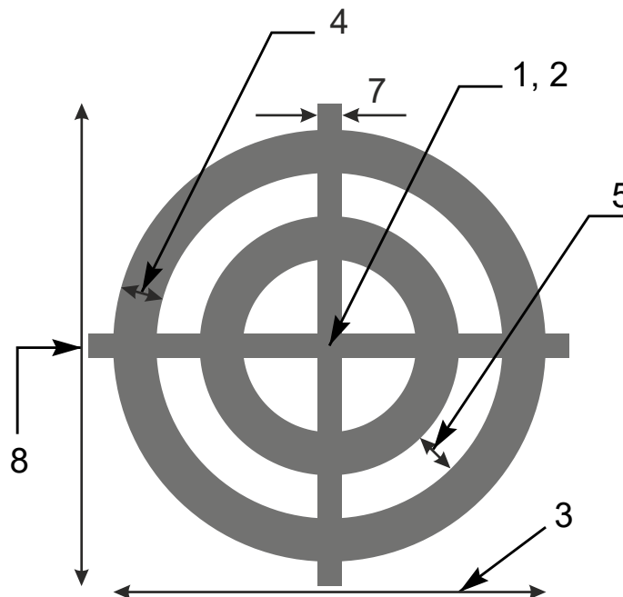
2. Moiré primitive
