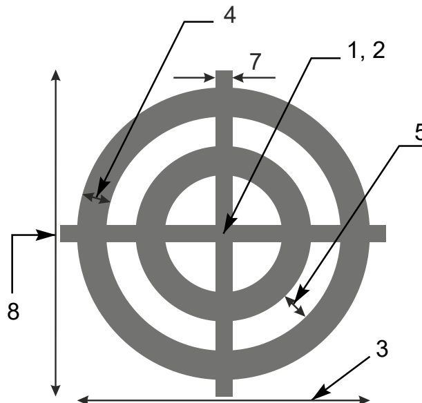
2. Moiré primitive
